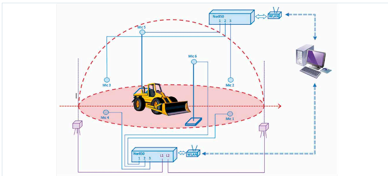
ISO 6395 setup
